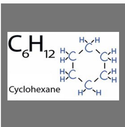
Cyclohexane
