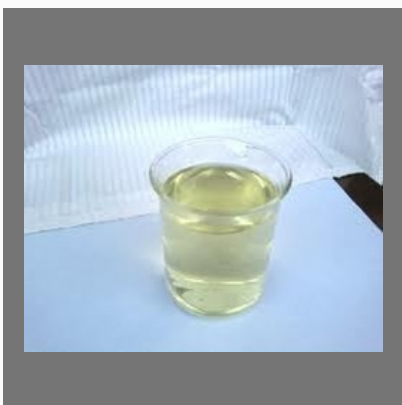
Triethylamine
