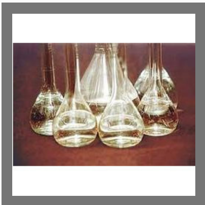
Epichlorohydrin Liquid
