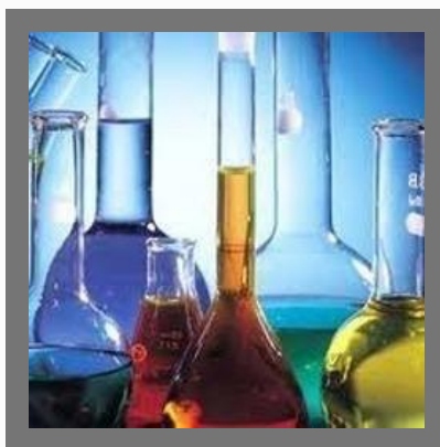
Isobutyric Acid
