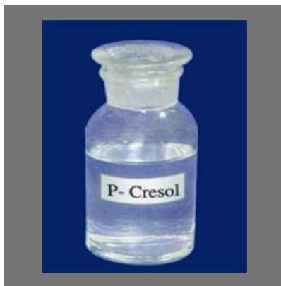
Paracresol 99.1
